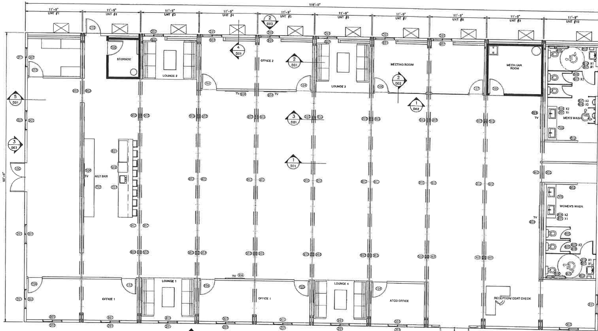
1 COMPLEX FLOOR PLAN A01 3/16"=1'-0"
